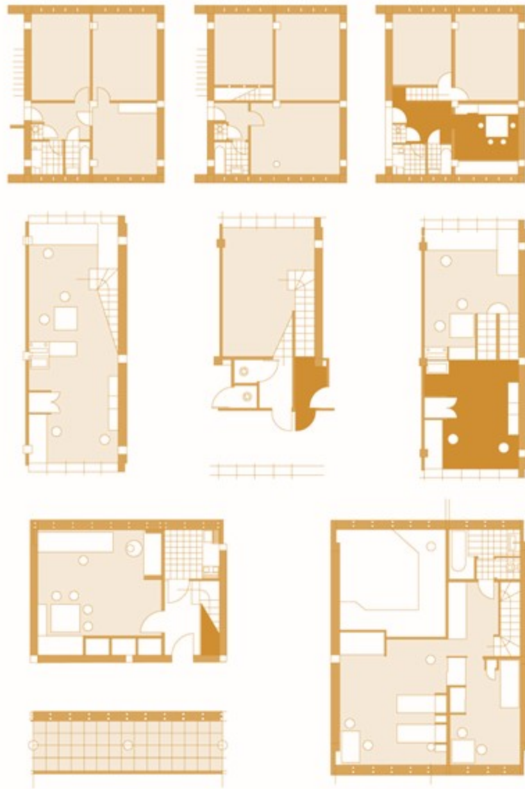
Narkomfin. Private space plans.
